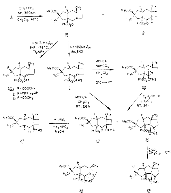
Scheme V
