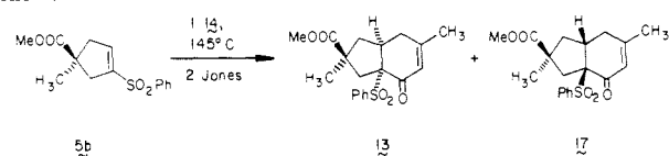
Scheme IV
