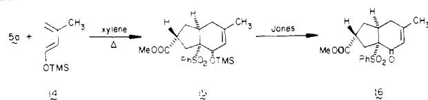
Scheme IV
